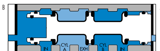
2 POS. DOUBLE OPERATOR B ACTUATED SHOWN
